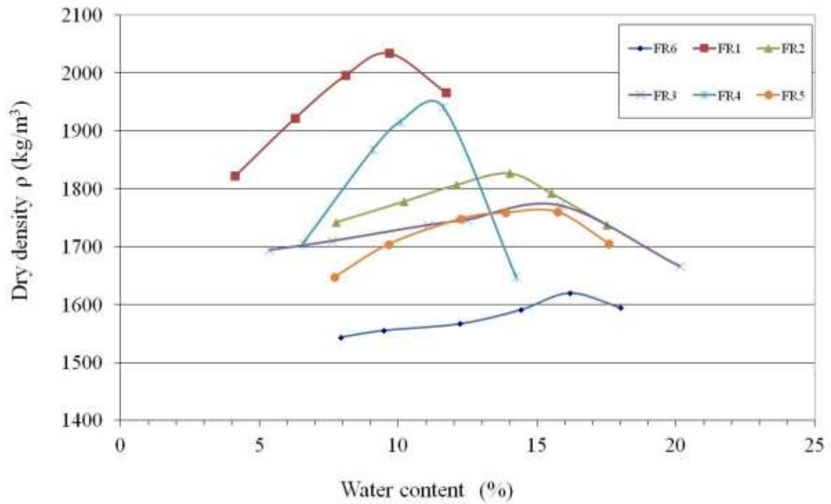
Figure 2. Proctor curves of FR soils
