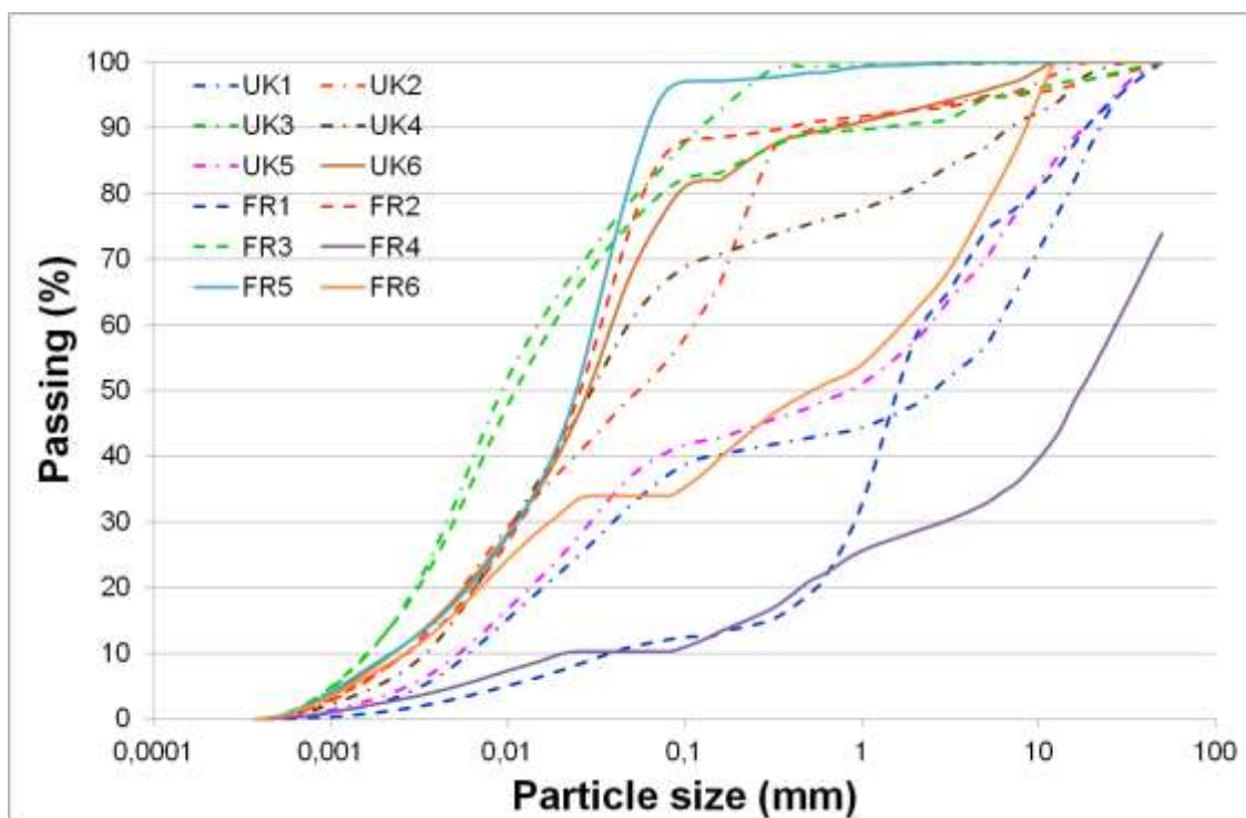
Figure 1. Soils particle size distribution
